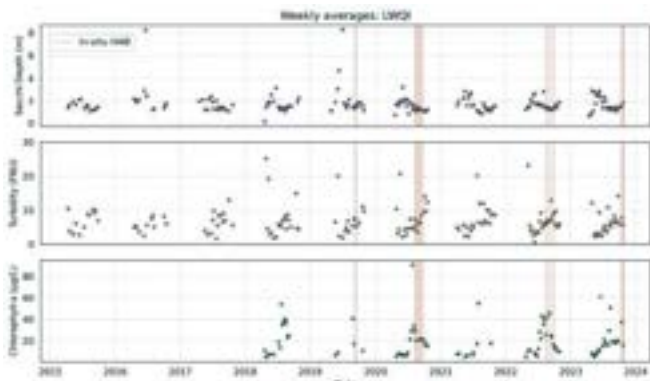
Timeseries plots for Secchi depth, turbidity and chlorophyll-a in Devils Lake, 2018-2023.
