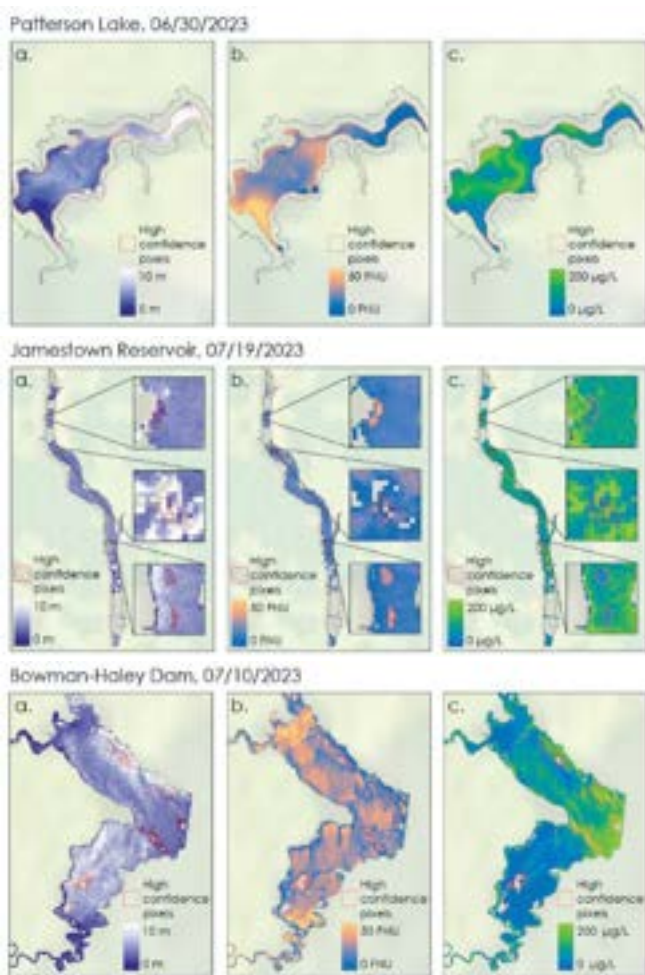
Snapshots of spatial distribution of Secchi depth (left), turbidity (middle) and Chlorophyll-a (right) for Bowman-Haley Dam, Jamestown Reservoir and Patterson Lake.
