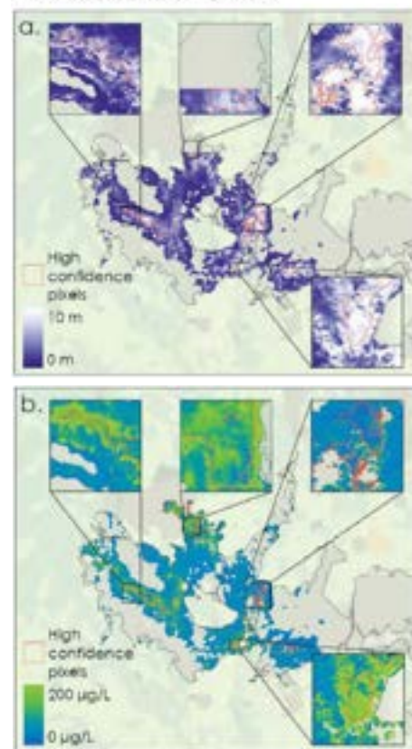
Snapshots of conditions on Devils Lake, a. Secchi depth and b. chlorophyll-a.
